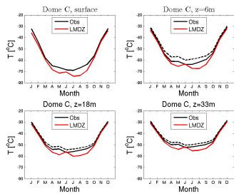
temp_DC_CM615-LR-amip-lwoff-00_1985_1994
