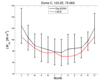
tsol_DC_CM615-LR-amip-lwoff-00_1985_1994
