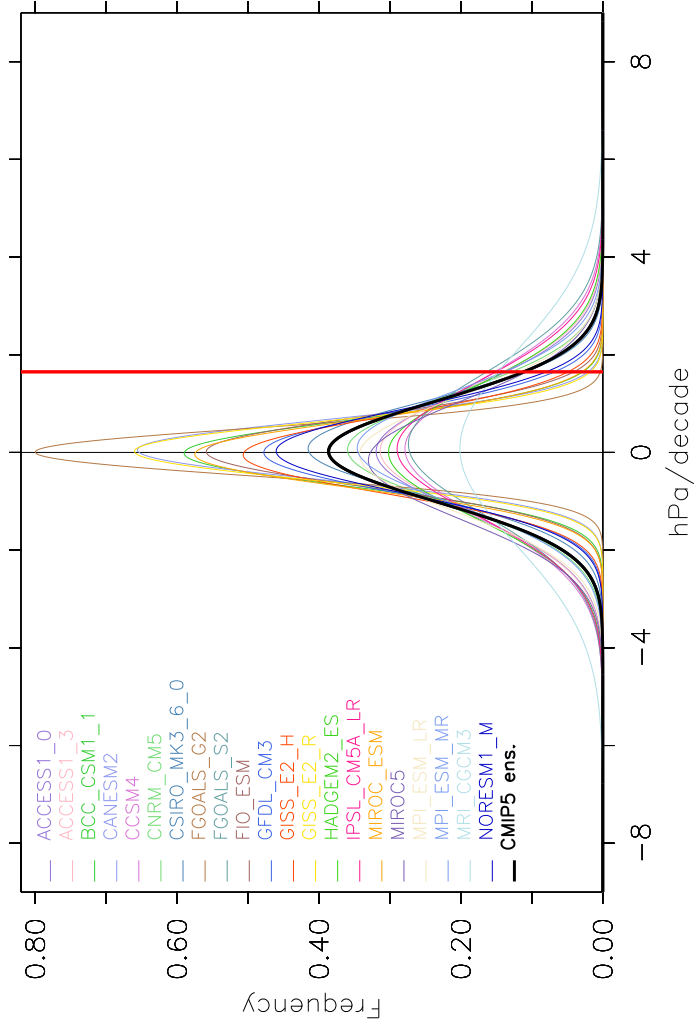
d) SAM 36-yr trend: piControl
