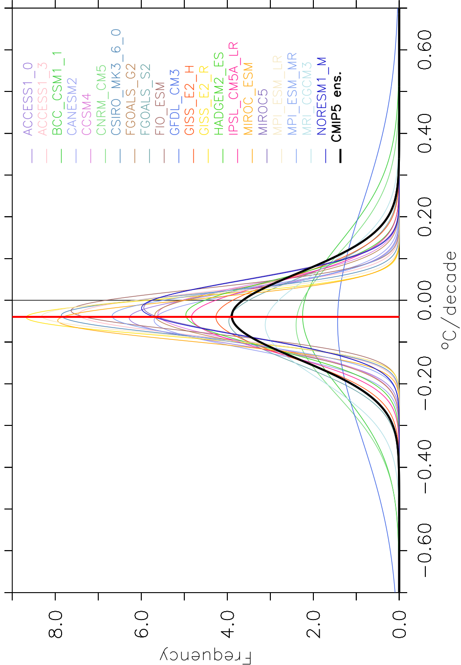
c) SAT 36-yr trend: piControl
