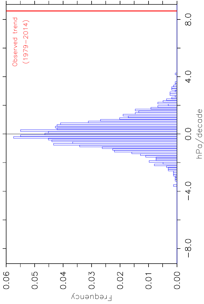
SAM 36-yr trend: CMIP5 piControl Ensemble
