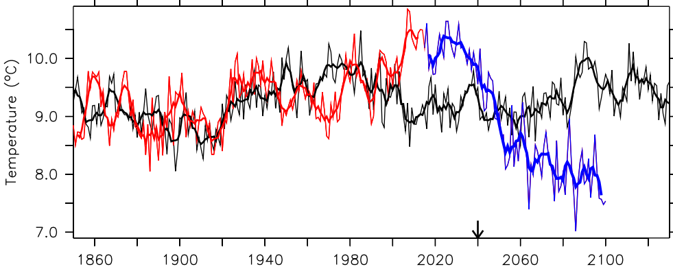
b) MRI-ESM2-0
