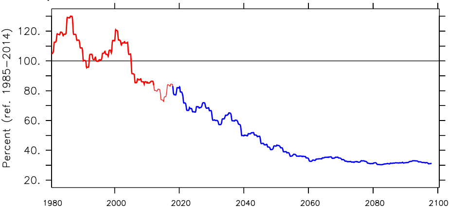
b) MRI-ESM2-0
