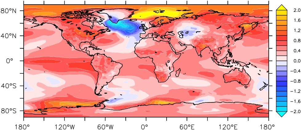
b) MRI-ESM2-0 [2040:2059]-[2020:2039]
