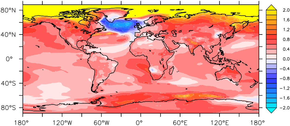
c) NorESM2-LM [2037:2056]-[2017:2036]
