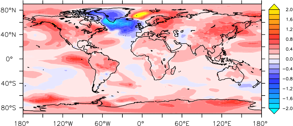
c) NorESM2-LM [2037:2056]-[2017:2036]
