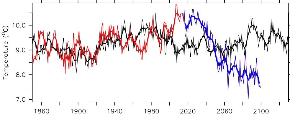
b) MRI-ESM2-0
