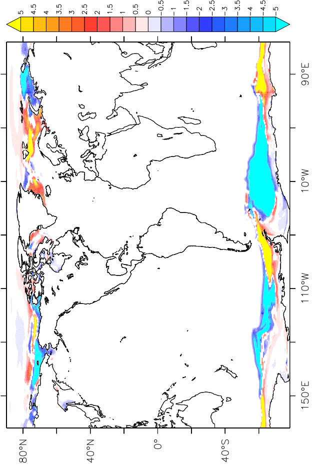
Regime 5, Threshold=2*std (<6 days), #Years=10/850
