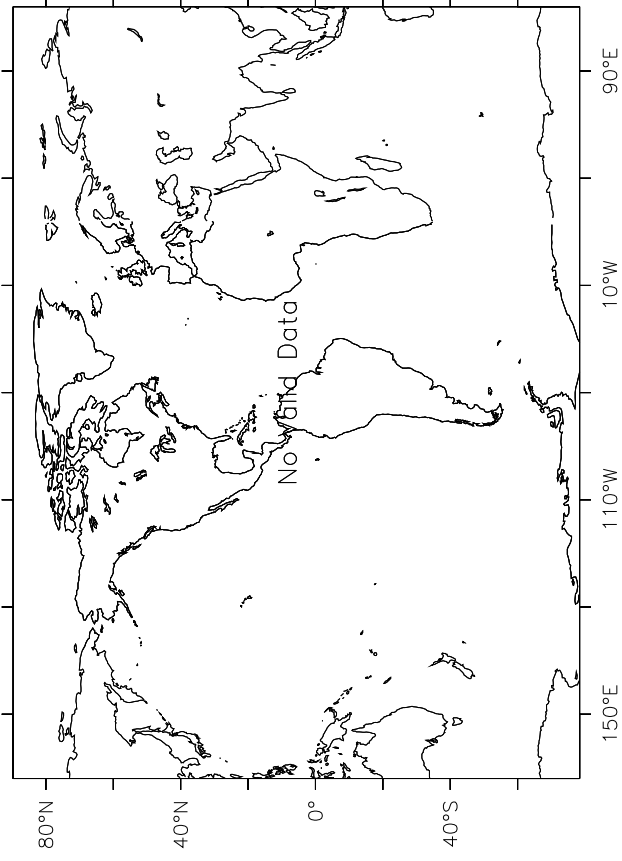
Regime 4, Threshold=2*std (<-6 days), #Years=bad/850
