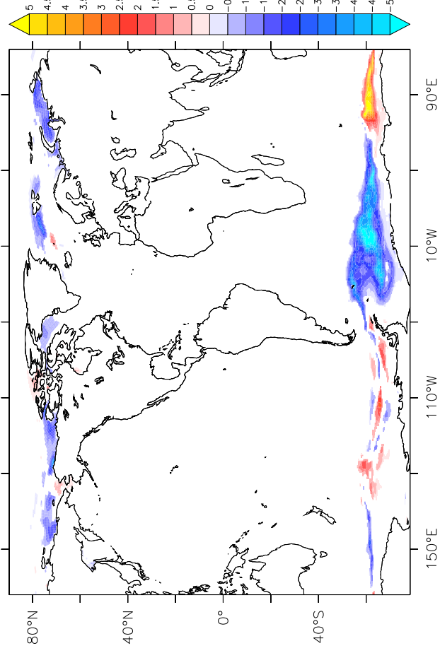
Regime 2, Threshold=1*std (<15 days), #Years=135/850
