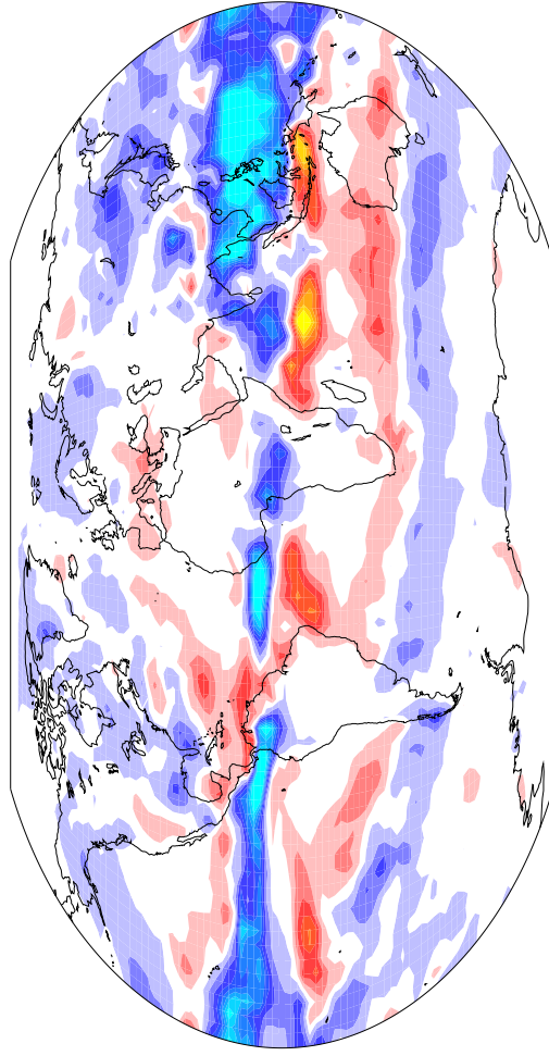
Ensemble Mean pr (jja)
