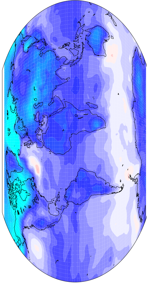
Ensemble Mean ts (djf)
