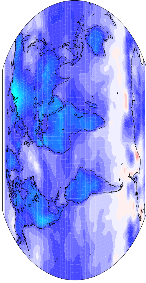
Ensemble Mean ts (jja)
