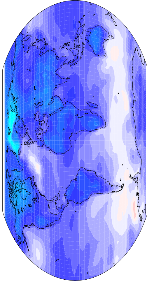
Ensemble Mean ts (ye)
