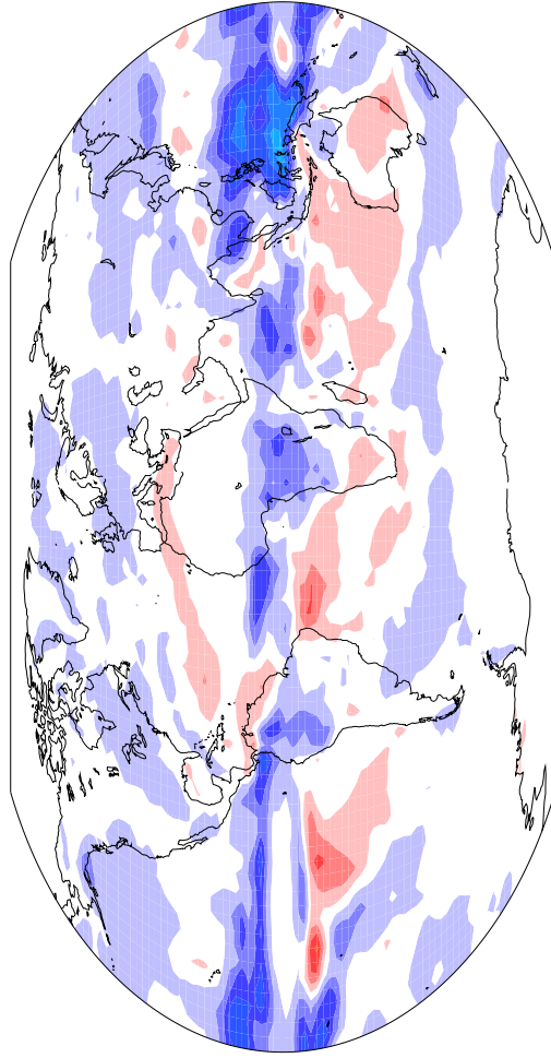
Ensemble Mean pr (ye)
