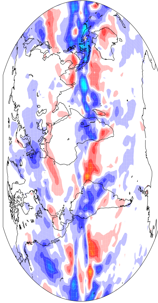
Ensemble Mean pr (djf)
