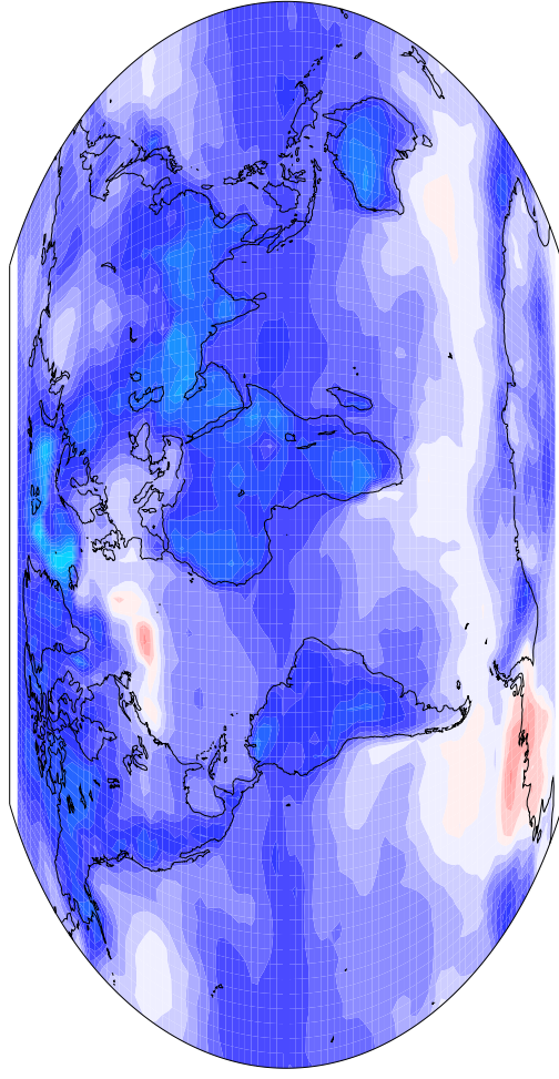
Ensemble Mean ts (mam)
