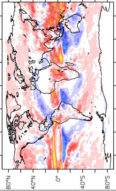
c) CCSM4
