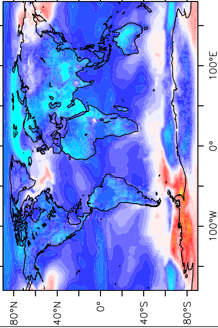
c) CCSM4
