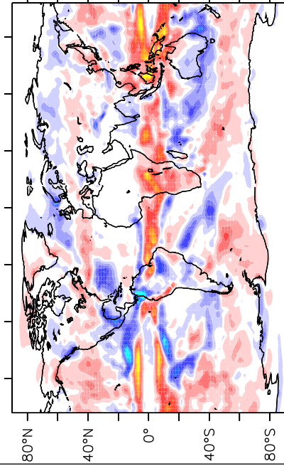
a) IPSL-CM5A-LR
