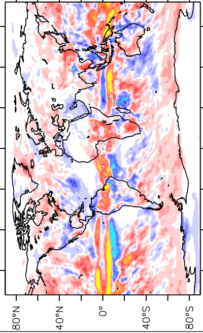
c) CCSM4
