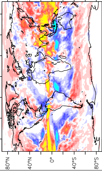
c) CCSM4
