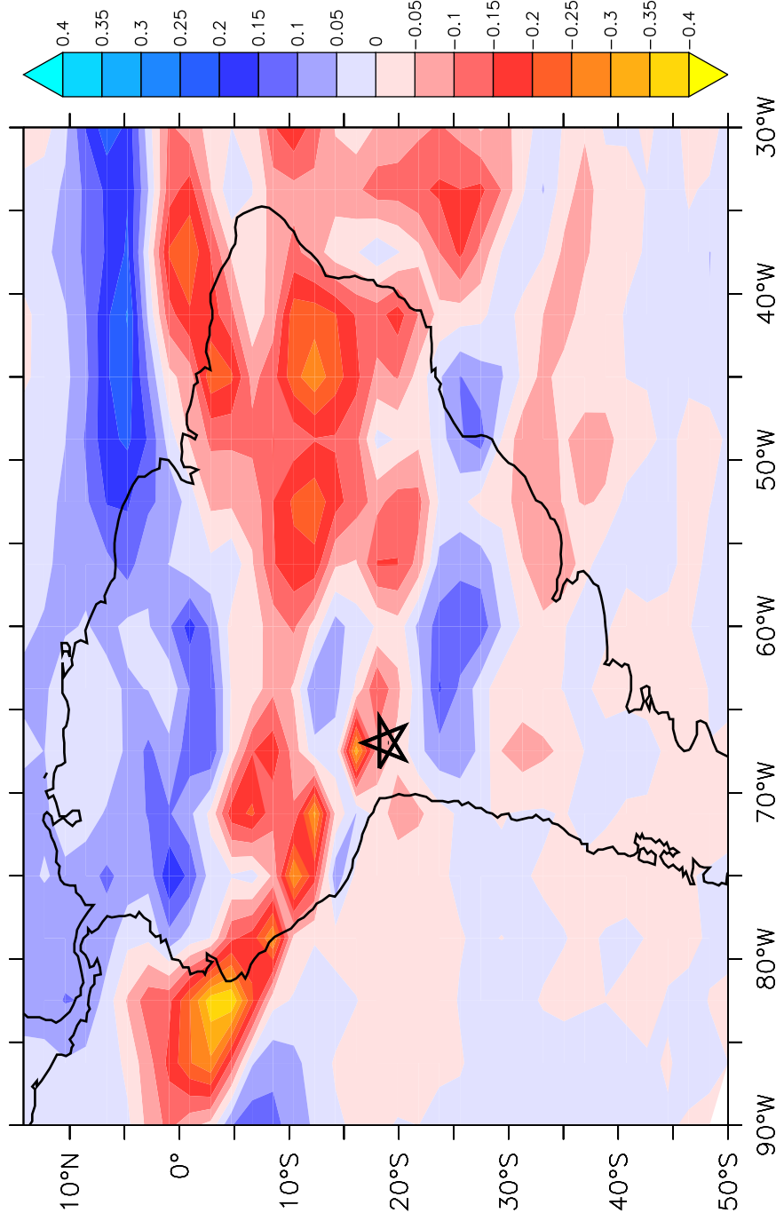
Precipitation anomalies (years:1210-1310)
