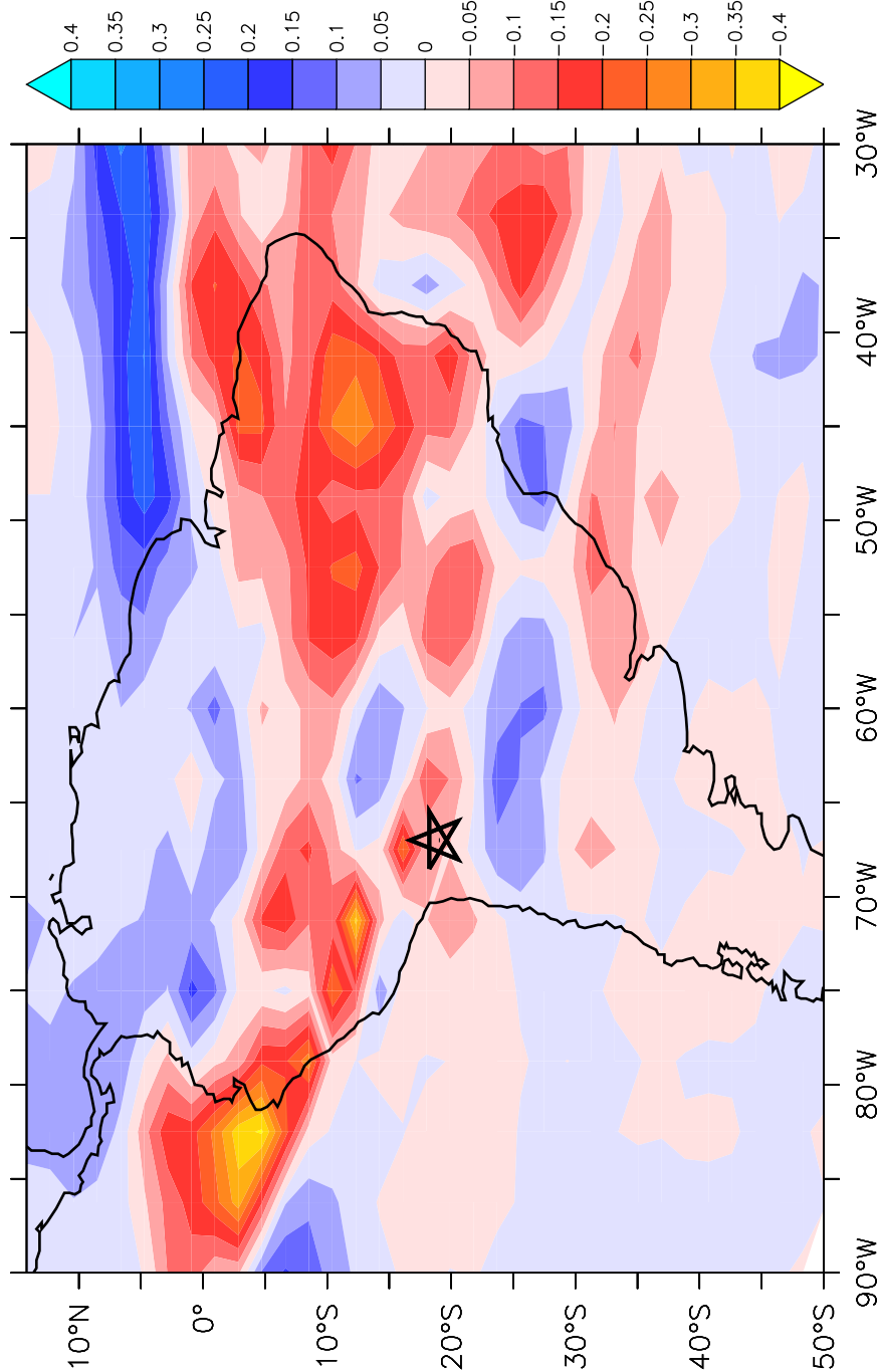
Precipitation anomalies (years:1200-1300)
