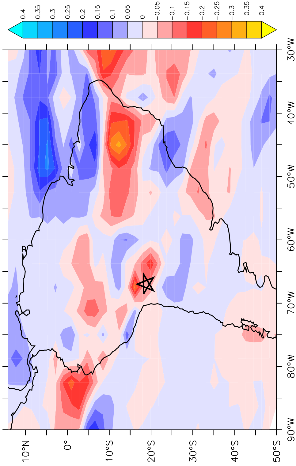
Precipitation anomalies (years: 1140–1240)
