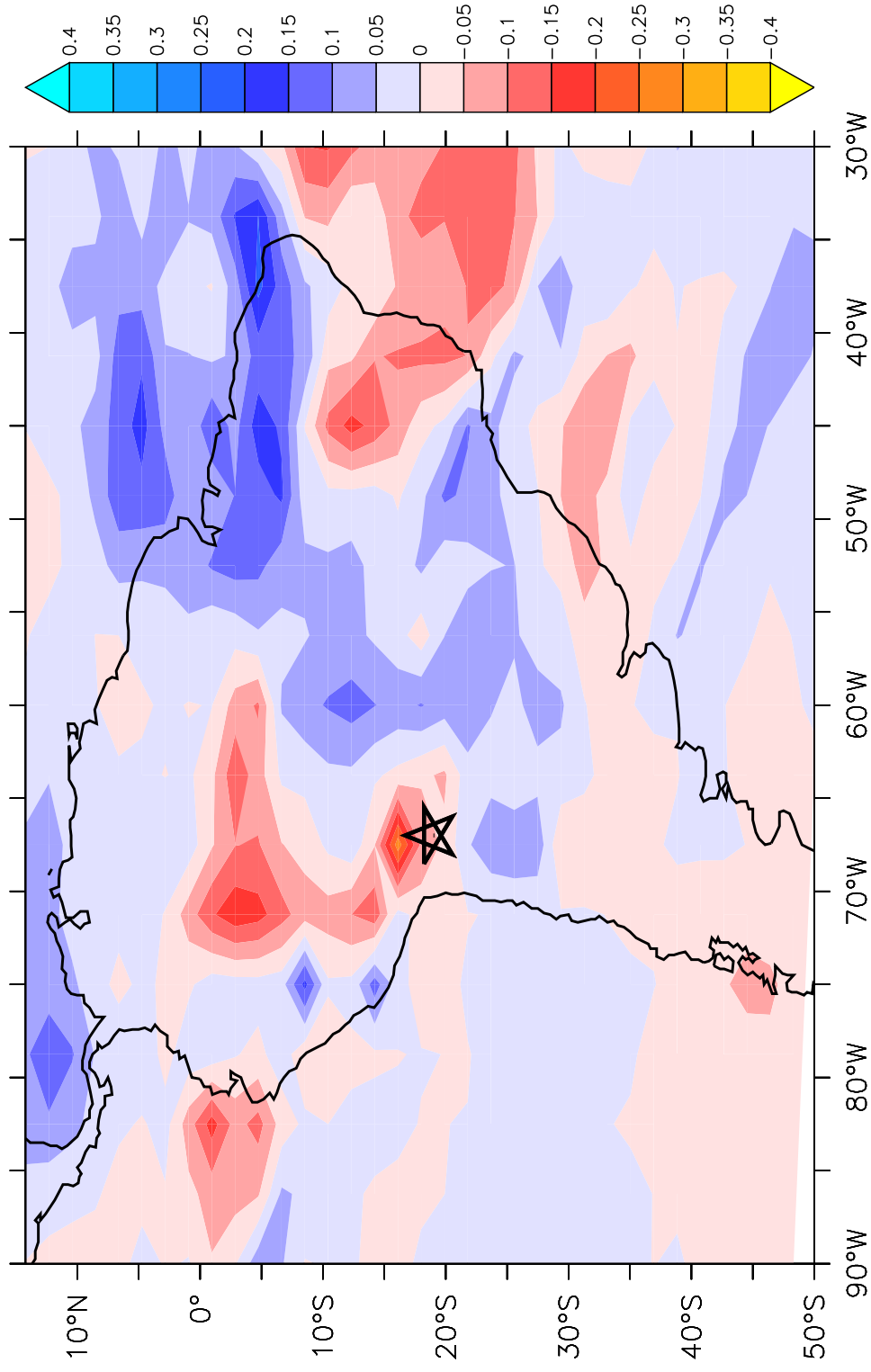
Precipitation anomalies (years: 1090–1190)
