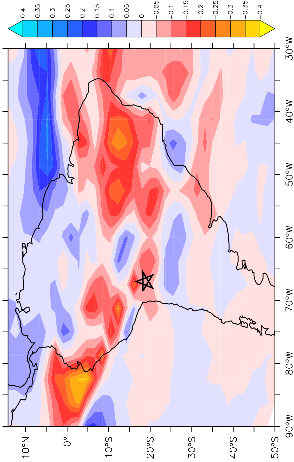
Precipitation anomalies (years: 1190–1290)
