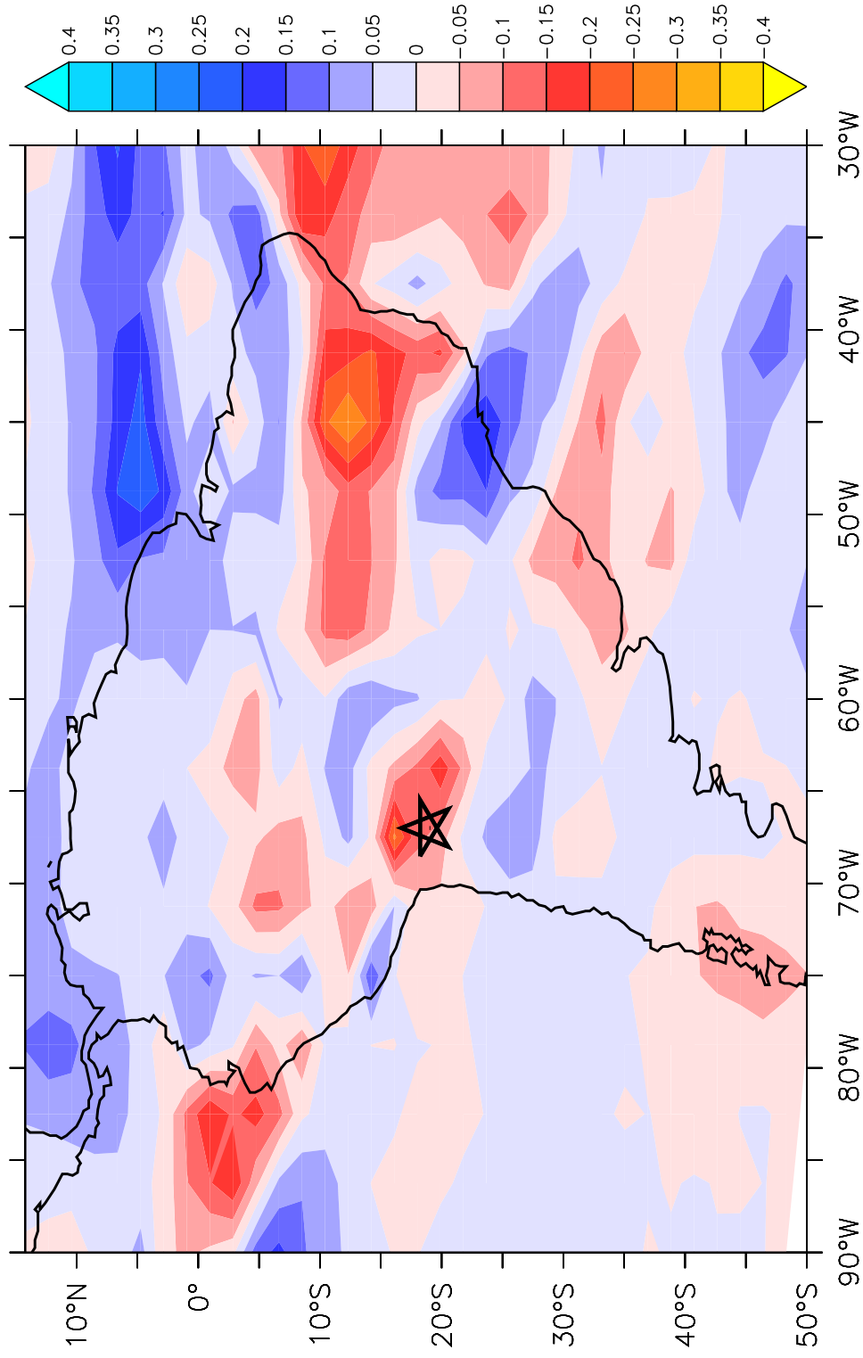
Precipitation anomalies (years: 1150–1250)
