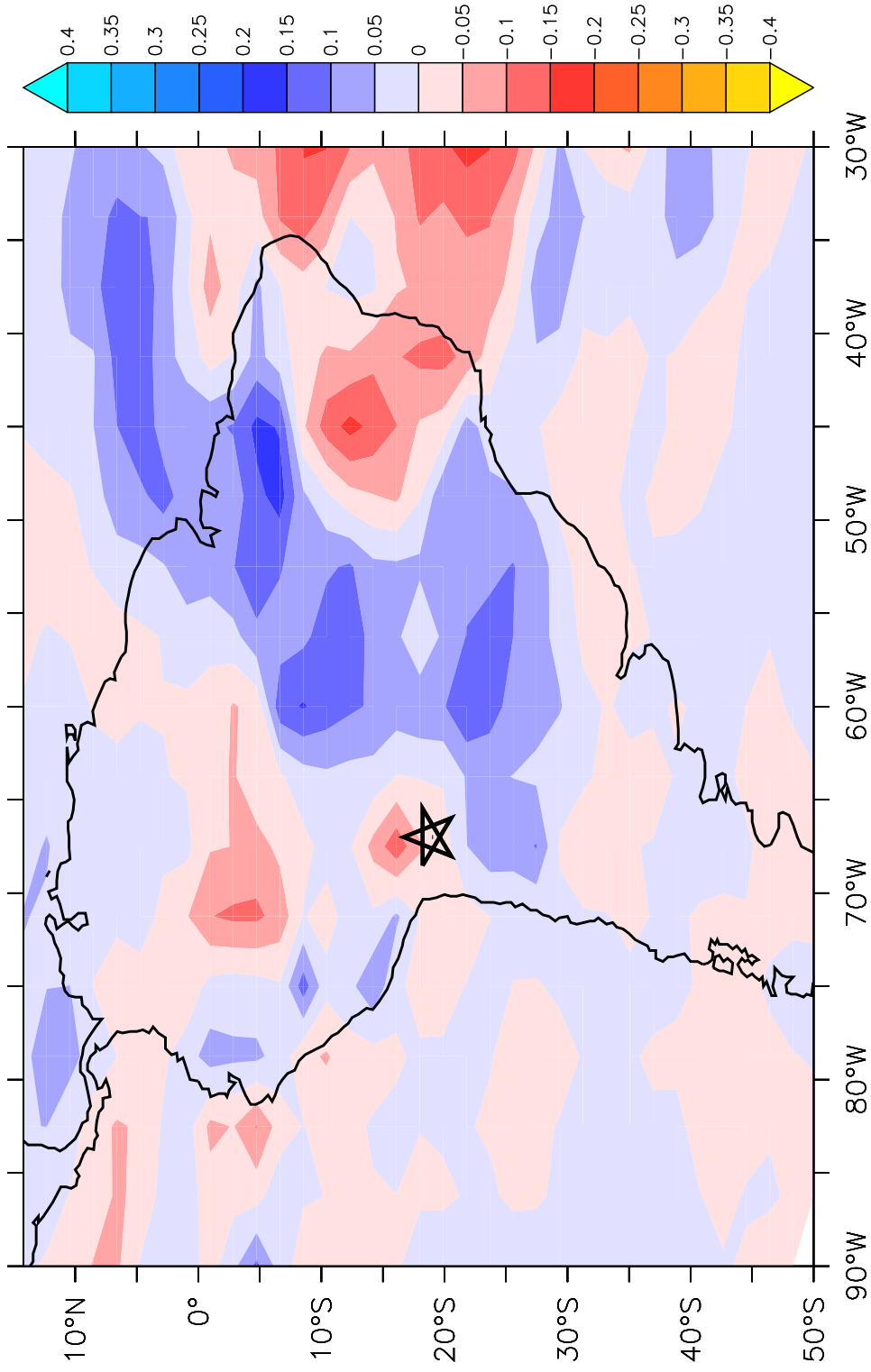
Precipitation anomalies (years:1060–1160)
