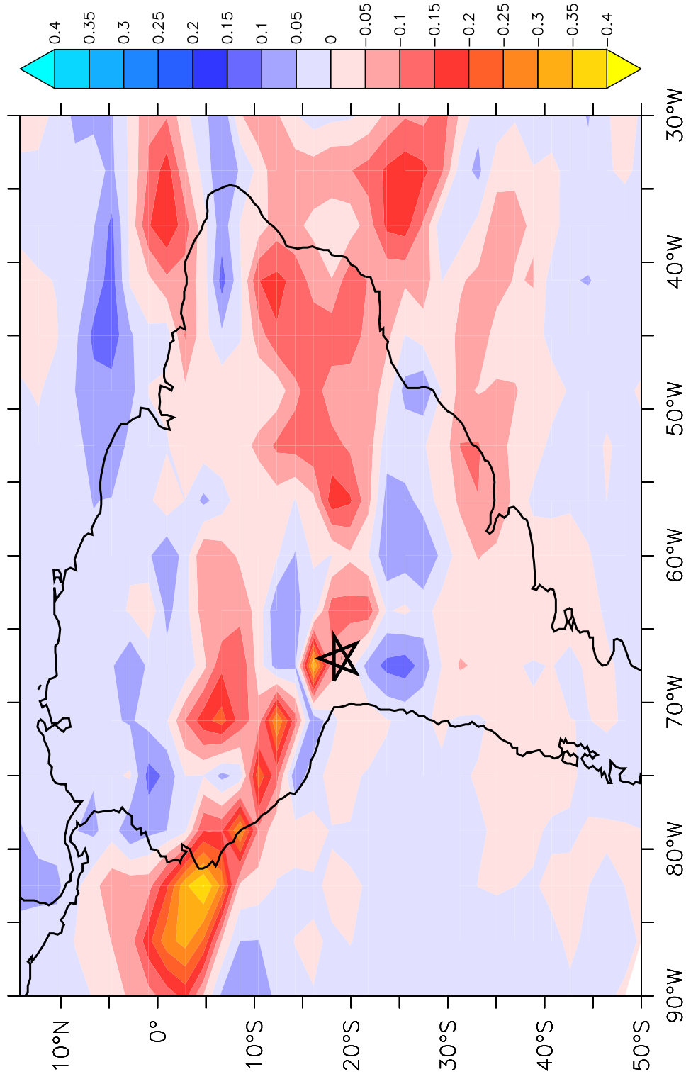
Precipitation anomalies (years: 1250–1350)
