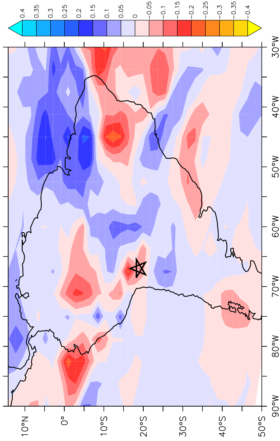
Precipitation anomalies (years: 1110–1210)
