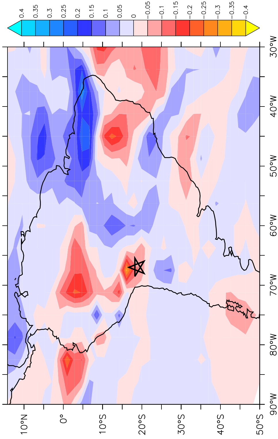
Precipitation anomalies (years: 1100–1200)
