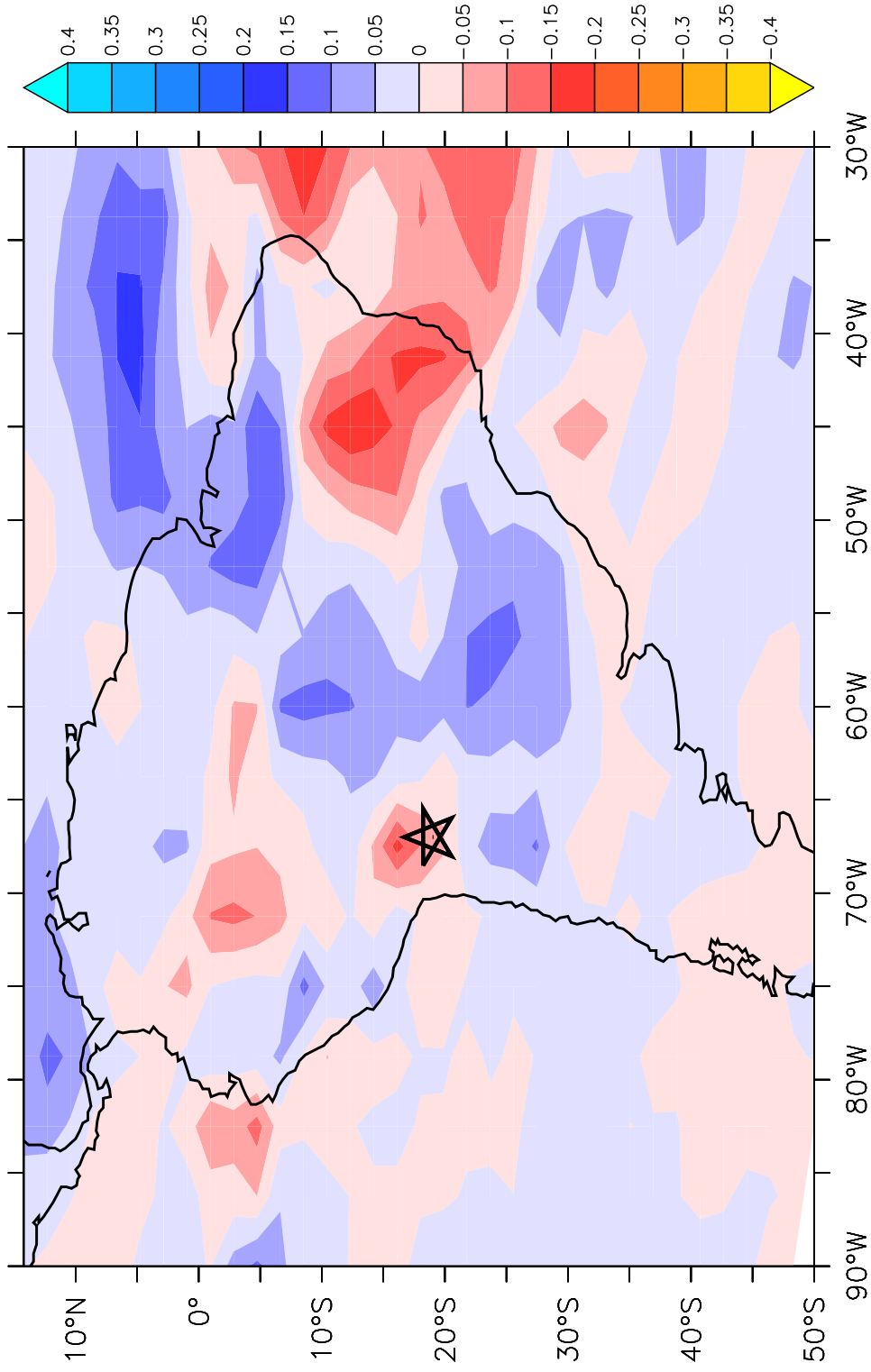
Precipitation anomalies (years:1070–1170)
