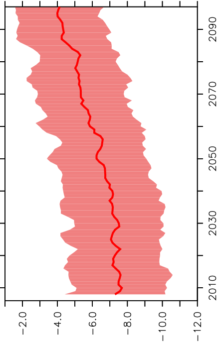
b) 2-meter temperature in RCP85
