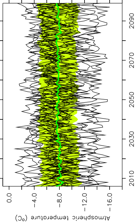
a) 2-meter temperature in RCP26
