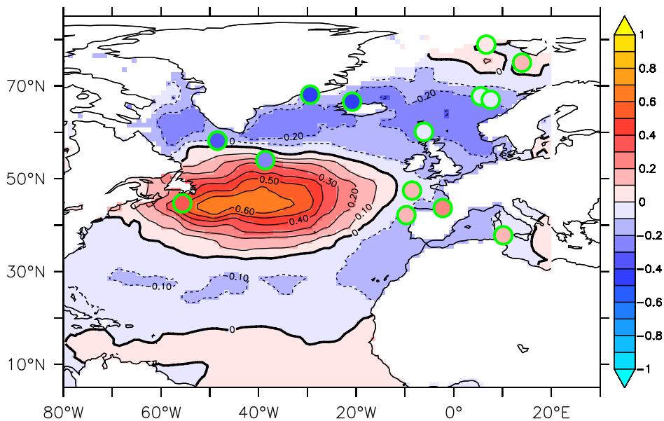
b) PC3 evolution ( r=0.31 )
