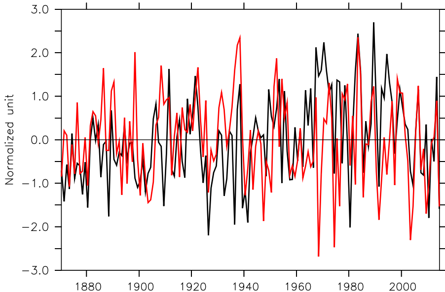
b) PC3 evolution ( r=0.31 )
