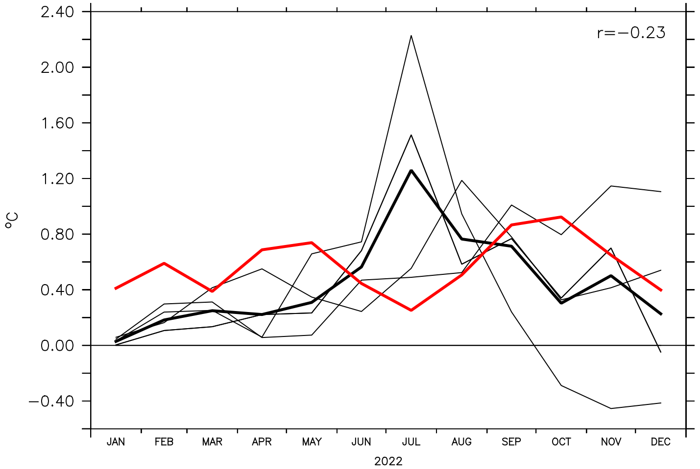
Euro-Atl sector
