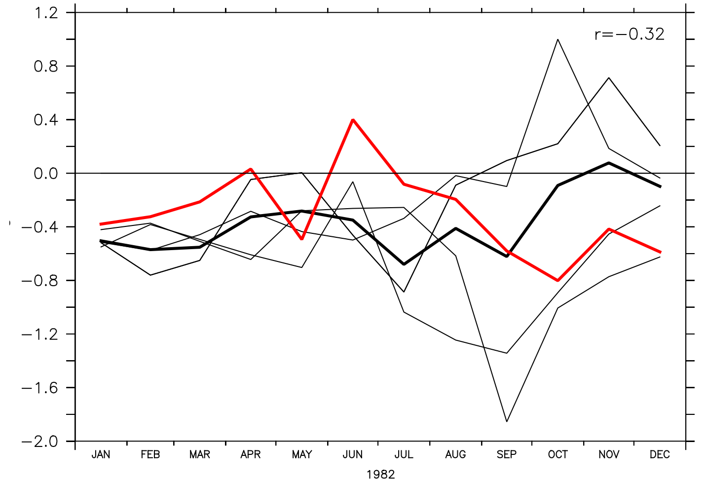
Biscay + UK
