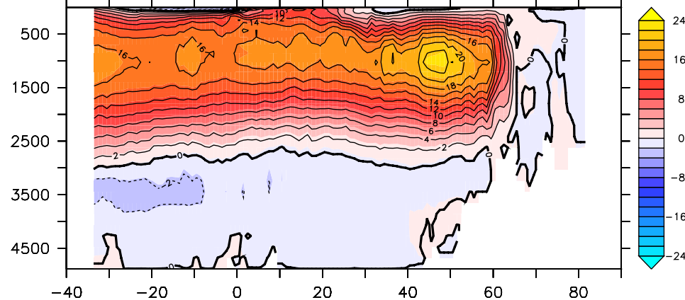
AMOC: yrs [2043–2089]–[2006–2041]
