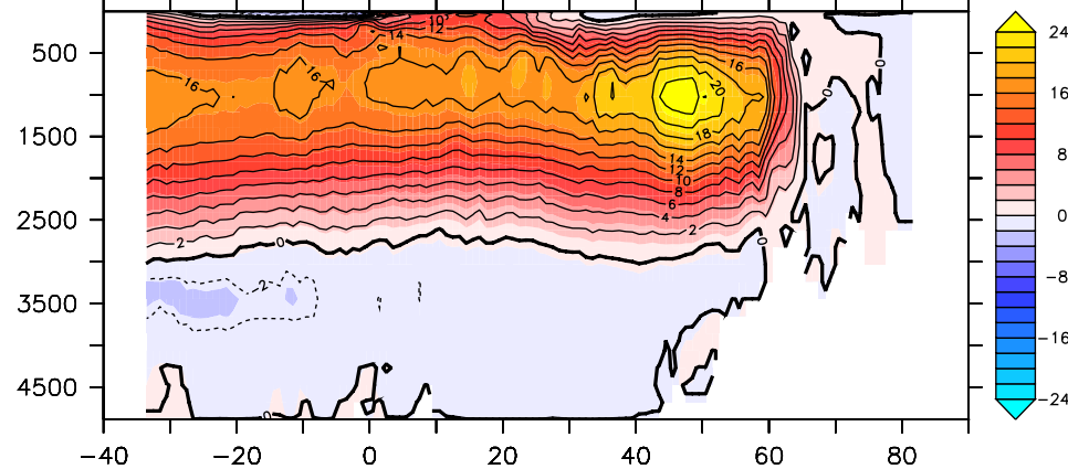
AMOC: yrs [2006–2041]
