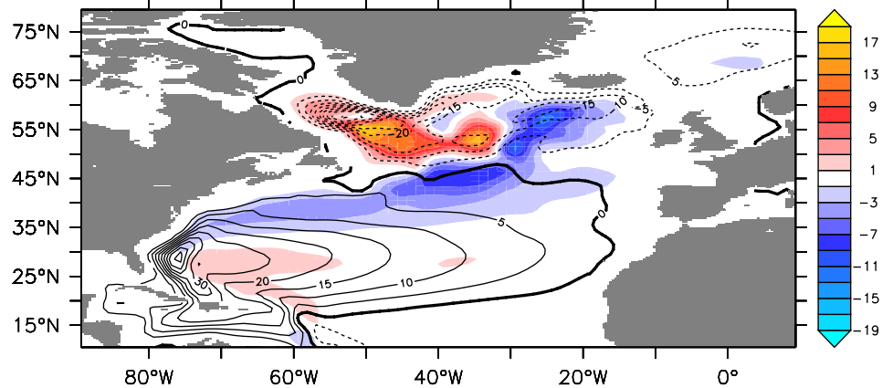
BSF: yrs [2043–2089]–[2006–2041]
