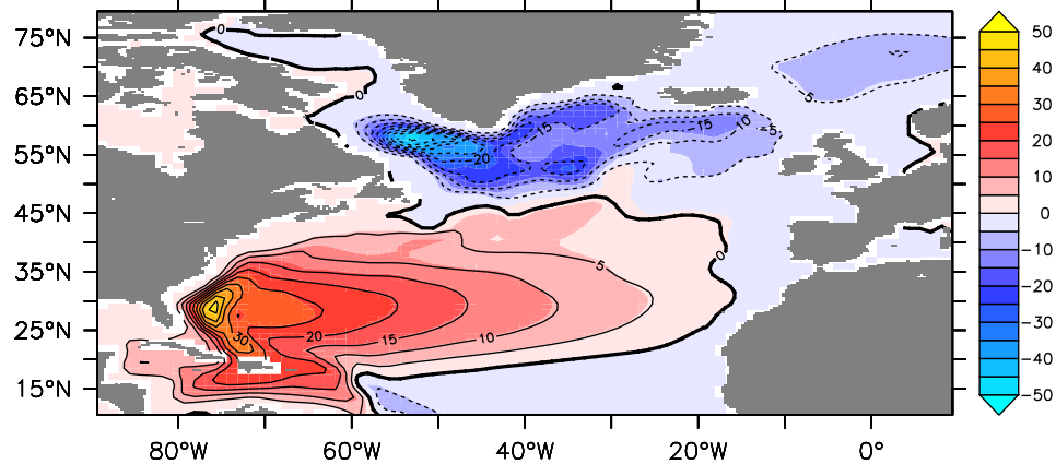
BSF: yrs [2043–2089]
