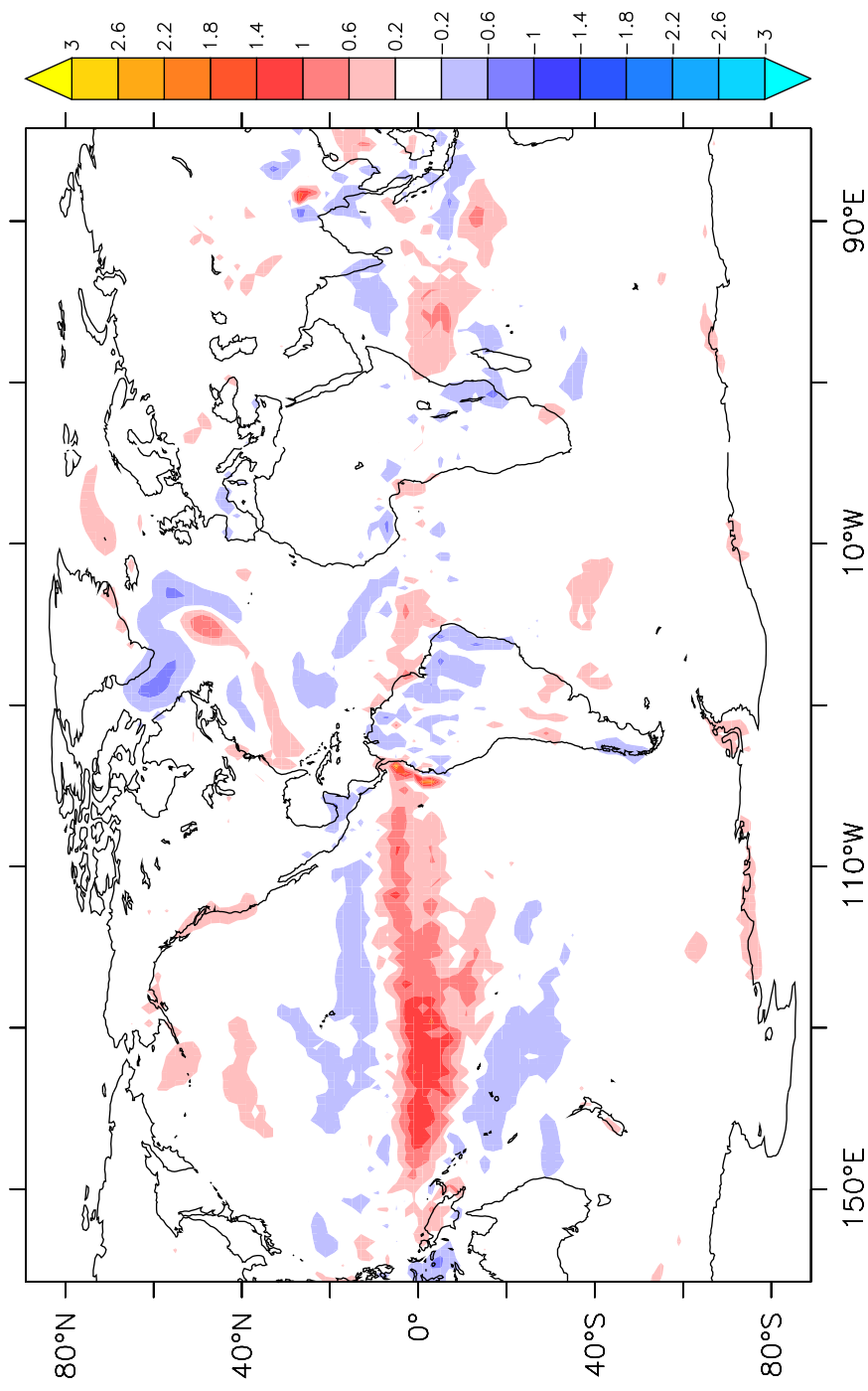
GISS-E2-R rcp26: [2055-2100]-[1950-2005]
