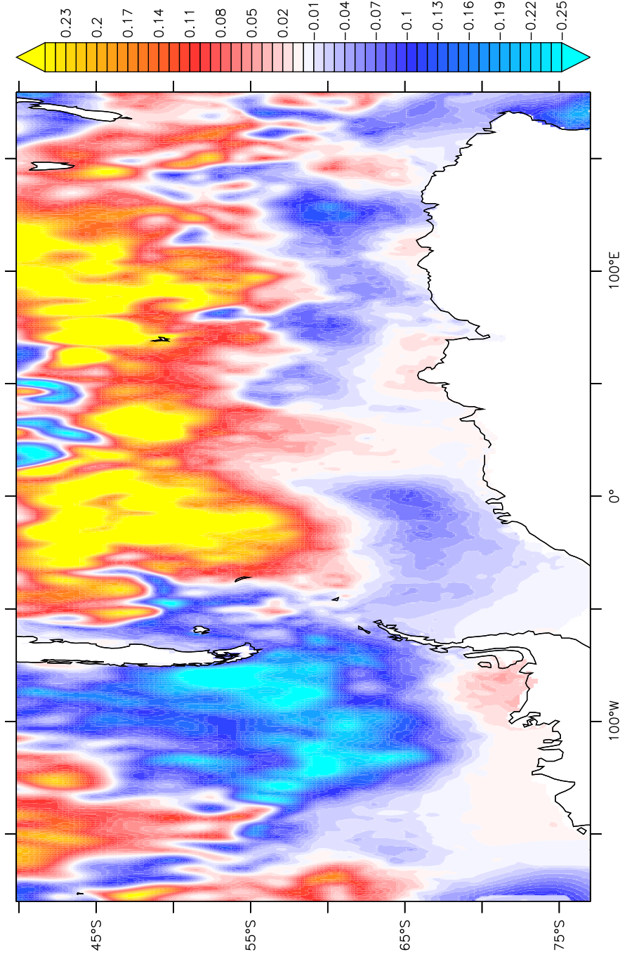
Mean SO surface temperature 2009–2012 ISAS
