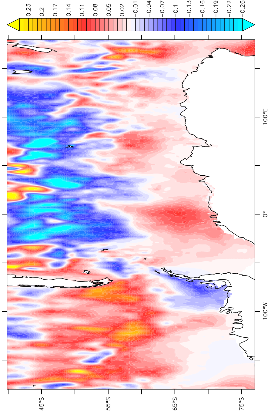
Mean SO surface temperature 2002 - 2005 ISAS
