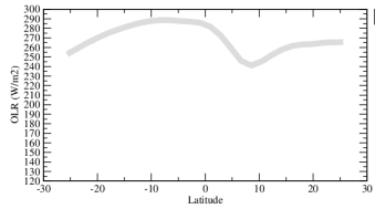
rlutzon
