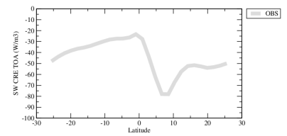
crestzon
