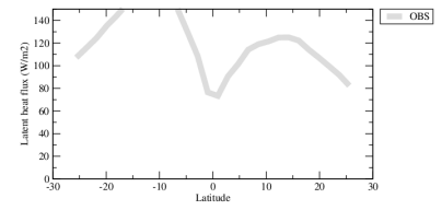
hflsazon
