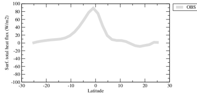
hfssazon
