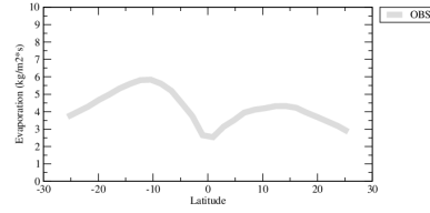
evazon
