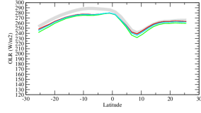
rlutzon
