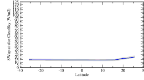
rsuscszon
