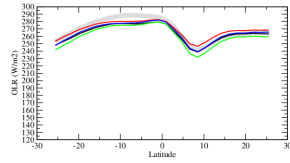
rlutzon
