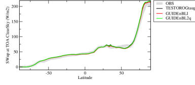
rsutczsn
