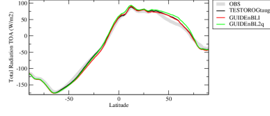
rttzcn
