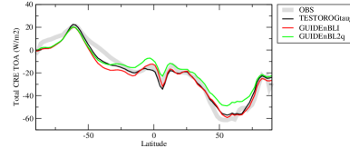
evazon
