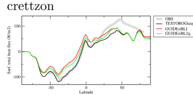
hfnzon
